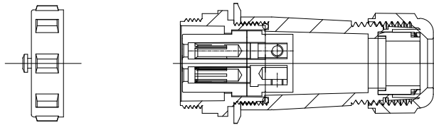
SECTION B-B
